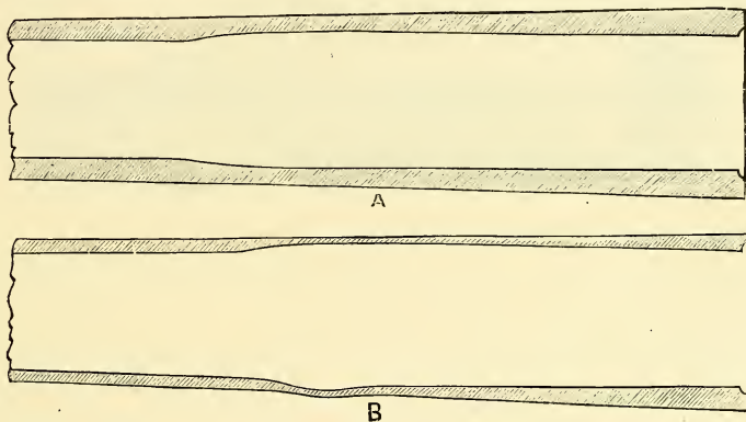
Section of Breech-end of Gun Barrels.
